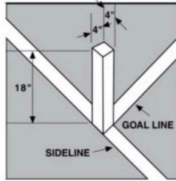
PYLON DETAIL
